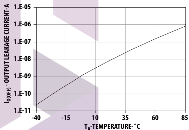
Figure 4. Typical Output Leakage vs Ambient Temperature
